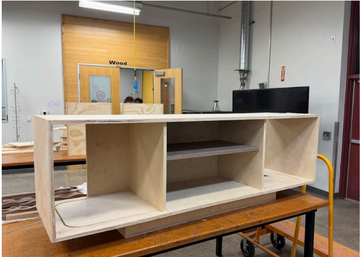
ASSEMBLING THE FULL CABINET. (NOTICE TAMBOUR GROOVES AND WALNUT SHELF) BASE INSTALLED.
